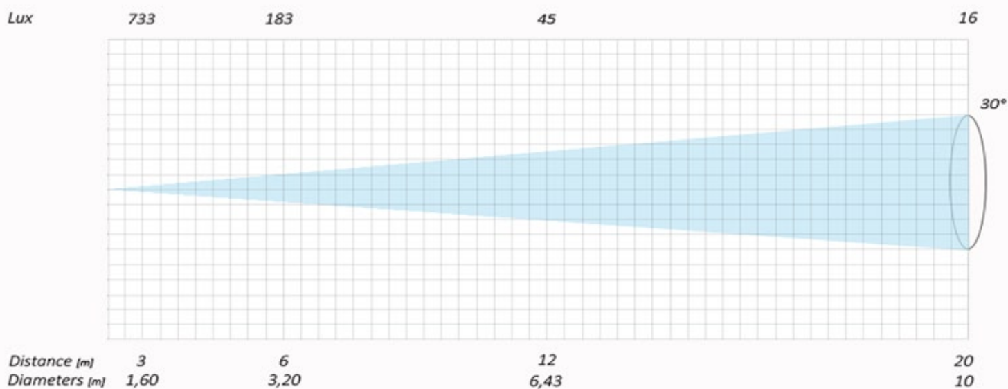
Goled Optic: 56mm
