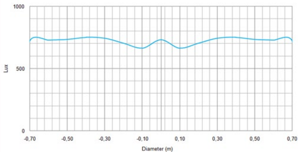
Goled optic 56mm Flux Output: 1.124 lm Distance 3 mt
