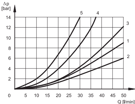
ELETTROVALVOLA COMMUTATA ENERGIZED VALVE
