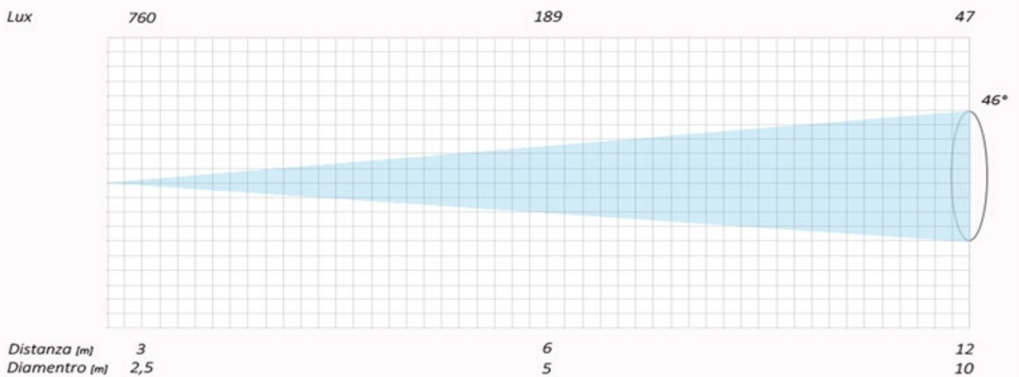
Golive 150 Optic: 56mm
