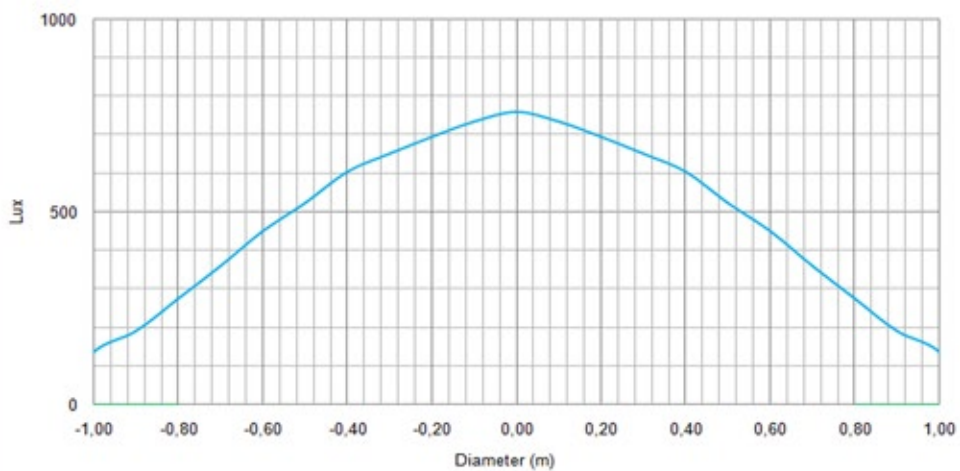
Golive 150 optic 56mm Flux Output: 1.194 lm
