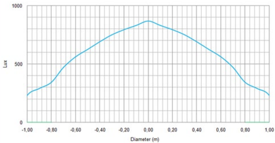
Golive 150 optic 115mm Flux Output: 1.496 lm
