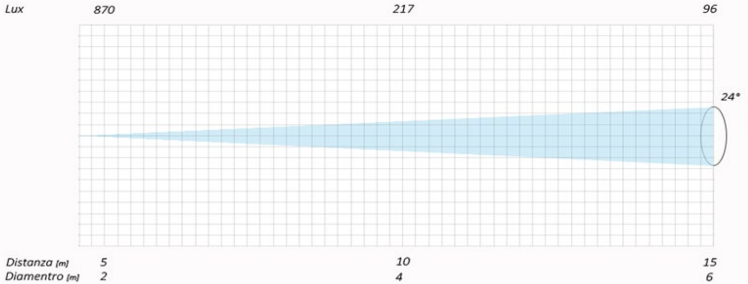
Golive 150 Optic: 115mm
