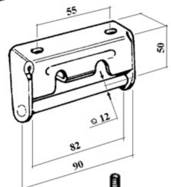
art. 15308 CERNIERA VIBERTI gr. 290
