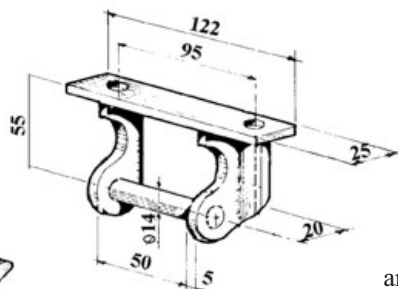
art. 15344 CERNIERA ALL.25 gr. 380
