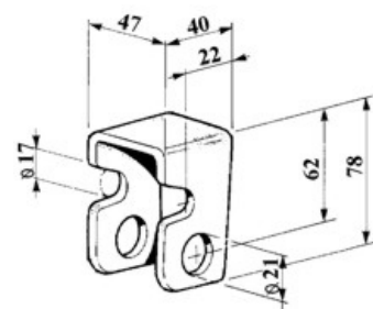
art. 15390 BUSSOLOTTO ALL.30 gr. 15
