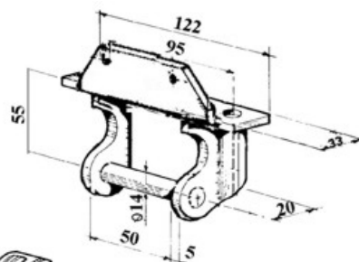
art. 15348 CERNIERA ALL.30 gr. 450
