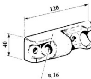
art. 15292 CERNIERA TIR PESANTE gr. 400
