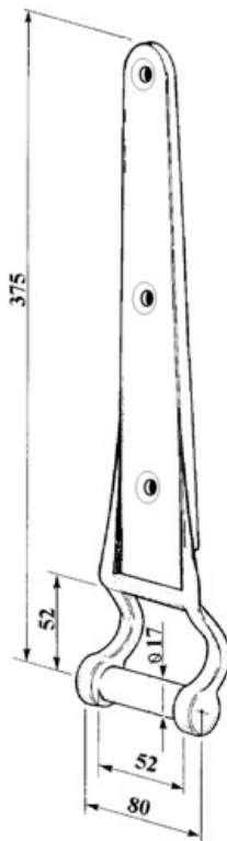
art. 15361 CERNIERA ALTA H375 gr. 1.050
