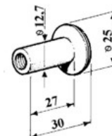
art. 15390 BUSSOLOTTO ALL.30 gr. 15
