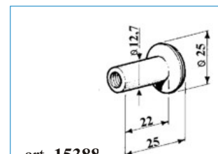
art. 15388 BUSSOLOTTO ALL.25 gr. 10
