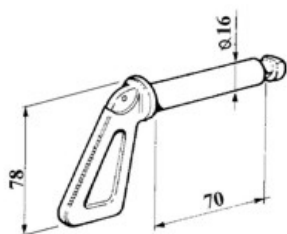
art. 15184 MANIGLIA STOPPED gr. 220
