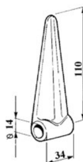
art. 15120 CERNIERA BOMBATA MEDIA gr. 170
