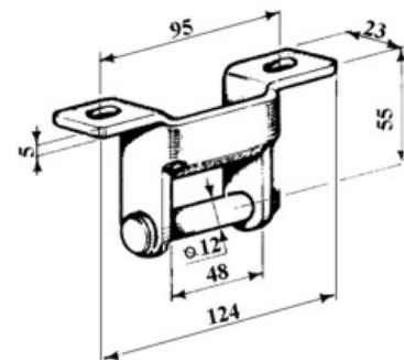
art. 15298 CERNIERA RAPID gr. 280
