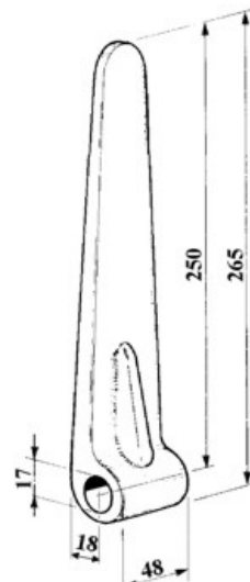
art. 15369 CERNIERA POST. H265 gr. 790
