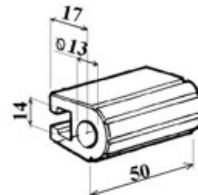
art. 15275 CERNIERA ALLUMINIO gr. 70
