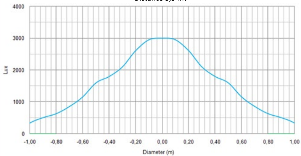
Golive 400 optic 56mm Flux Output: 3.385 lm Distance 3,5 mt
