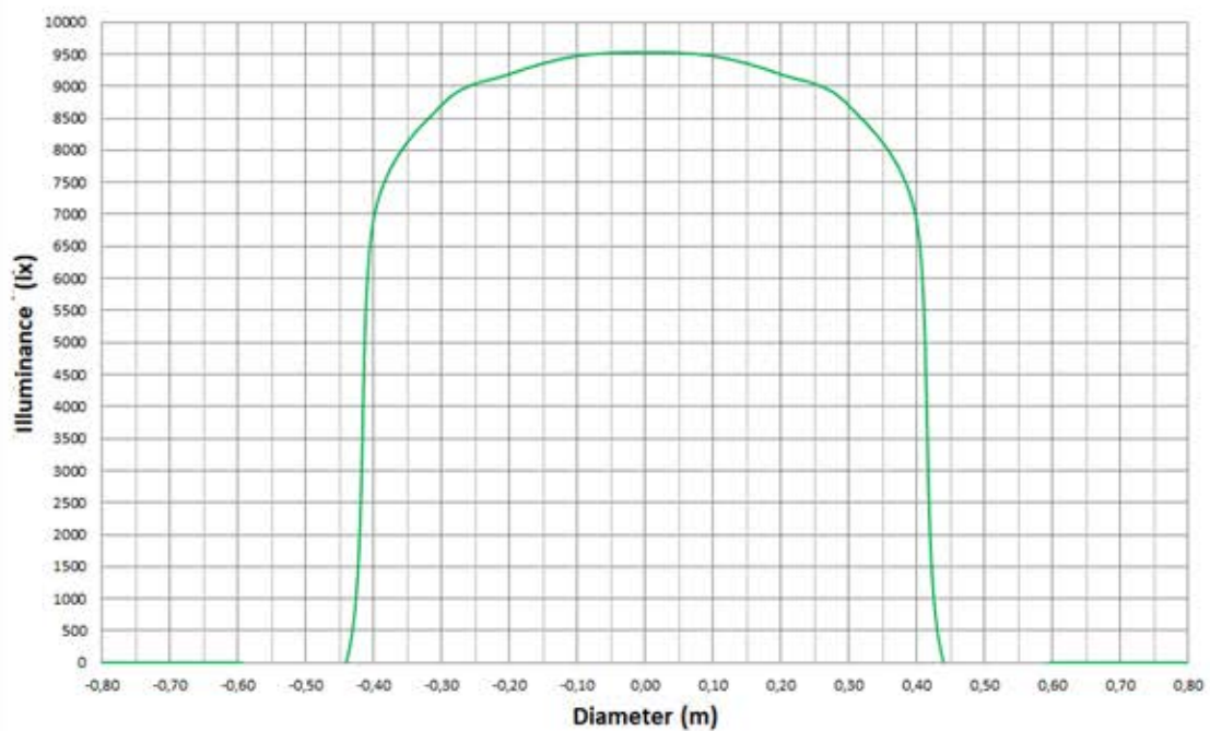
Signum optic 90mm Flux Output: 4278 lm Distance 2,5 m
